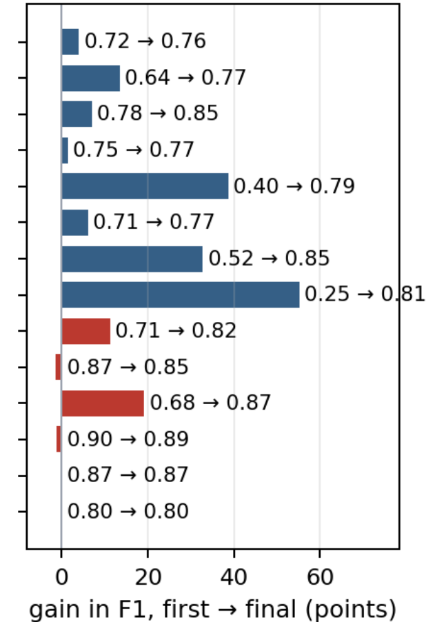
What the hours bought (Gemma-3-12B)
